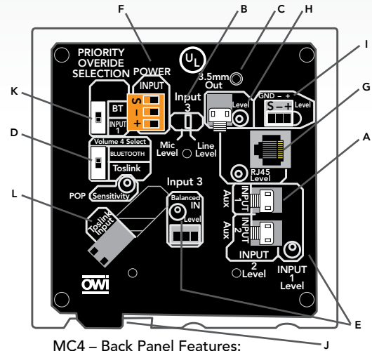
MC4 – Back Panel Features:
