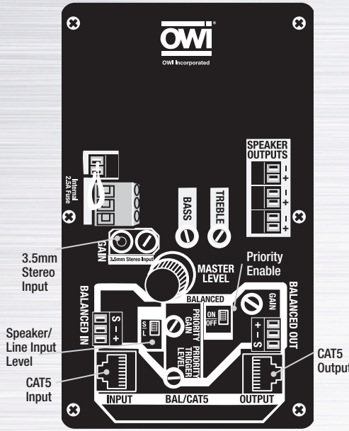
2X2-HD-IW83 2X2 FULL GRILL WITH HD AMPLIFIER
