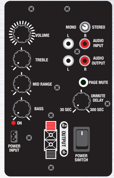
2X2-LV-IW83 2X2 FULL GRILL WITH LV AMPLIFIER
