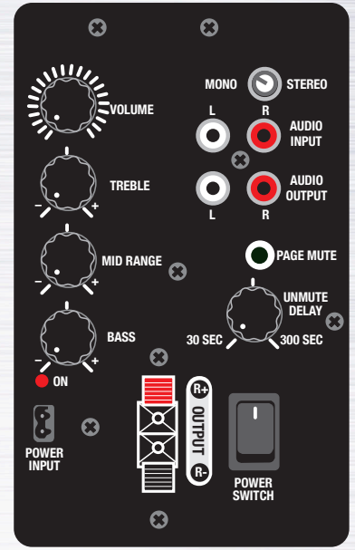
2X2-LV-IW63 2X2 FULL GRILL WITH LV AMPLIFIER
