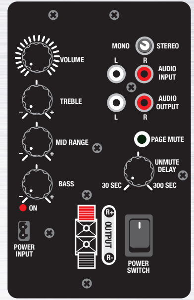
2X2-LV-IW62 2X2 FULL GRILL WITH LV AMPLIFIER
