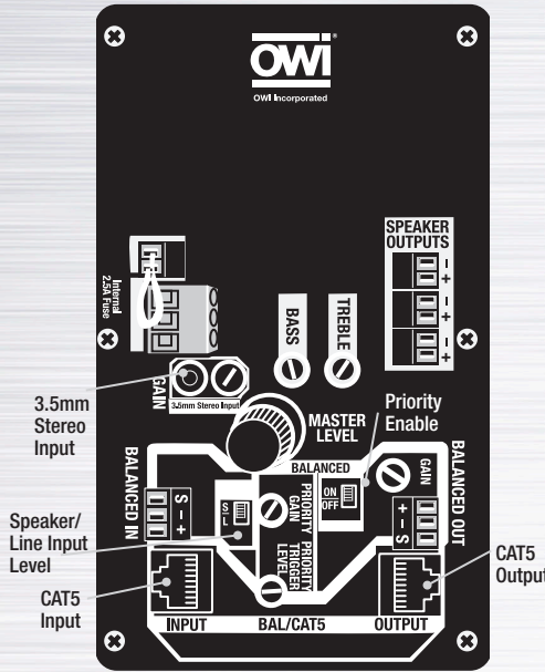
2X2-HD-IW63 2X2 FULL GRILL WITH HD AMPLIFIER
